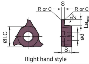
QC** turning/milling insert
